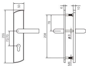
ABLOY® INOXI 3-19/012/120 PZ+PZ
